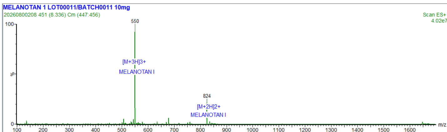
MASS SPECTRUM / SPECTRA
