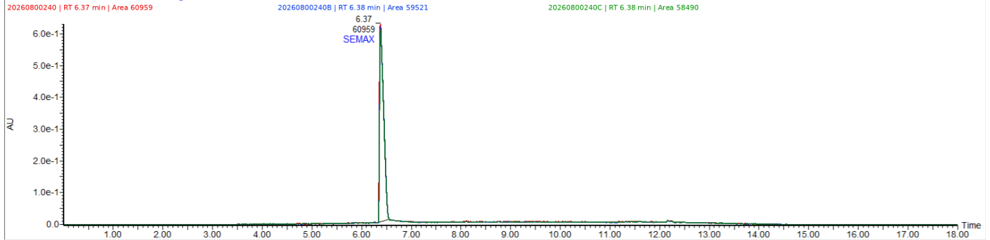
UV CHROMATOGRAM
